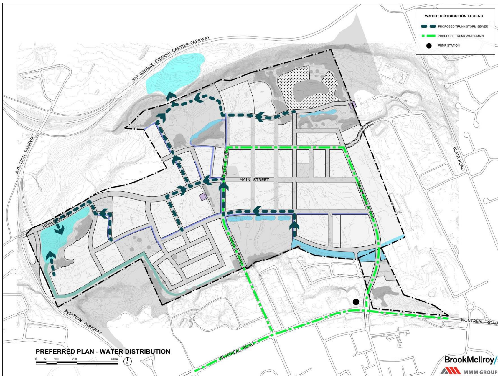
Figure 5.14 Water Supply
