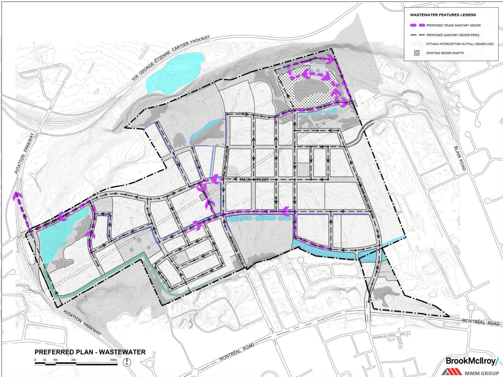
Figure 5.15 Wastewater
